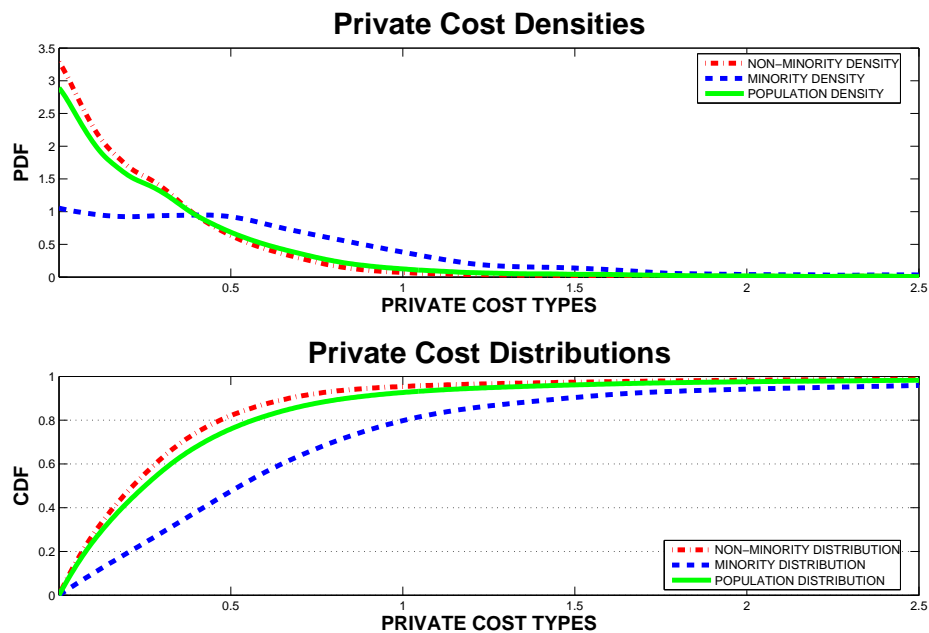
Figure 3.6: Type Distributions
